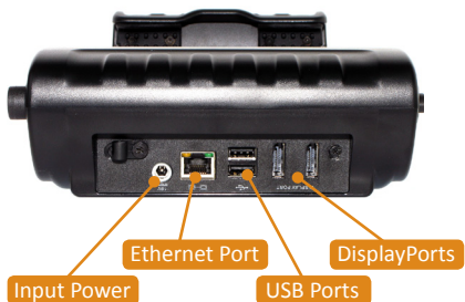
DT301/ DT311 Wall/ Vehicle Mount Cradle Bottom-view
