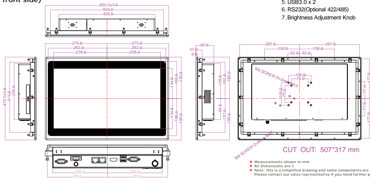
Real Flat Panel Mount (IP65 front side)
